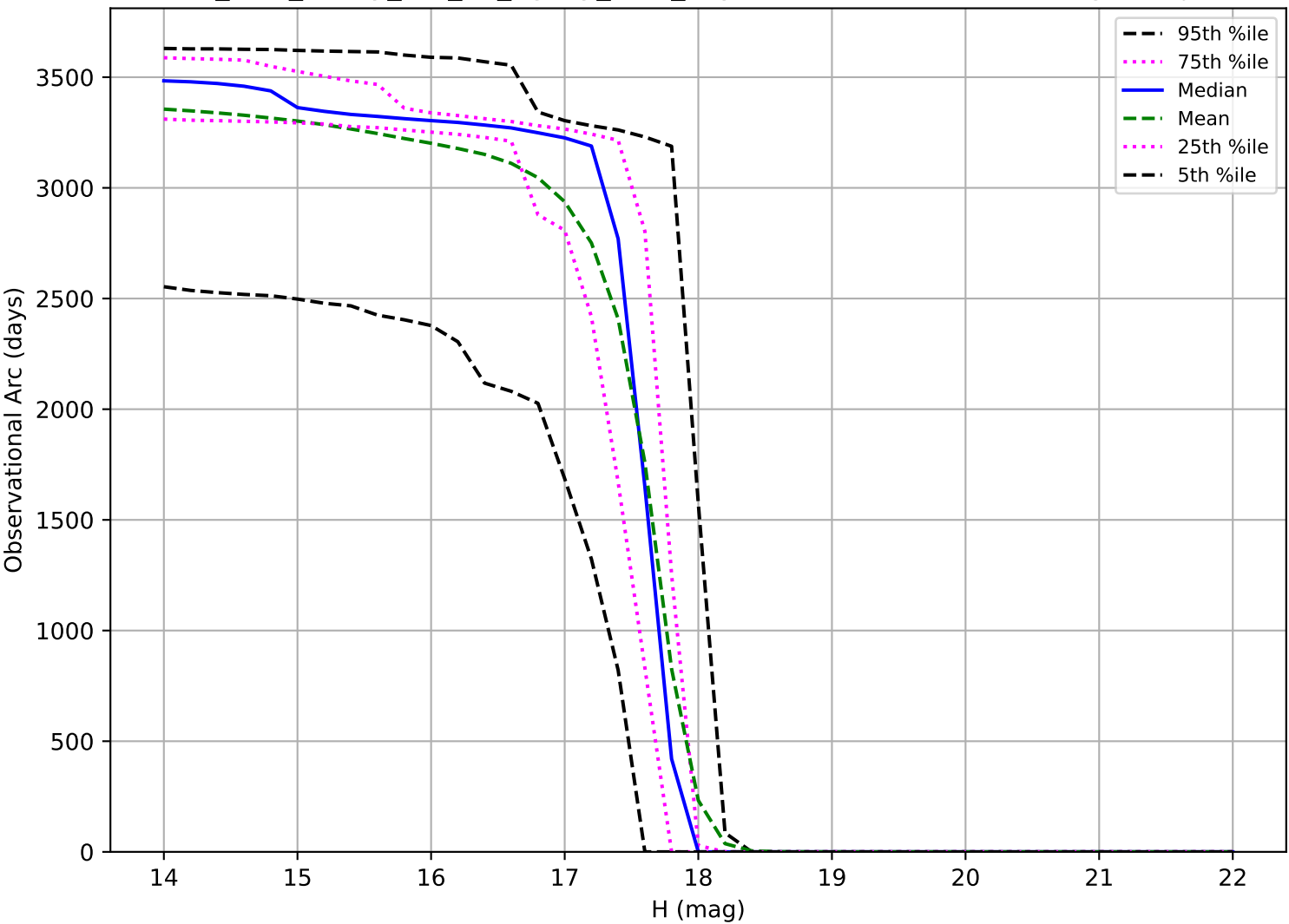
too_elab_heavy_r32_d2_ugrizy_v3.4_10yrs: Observational Arc Length Trojan
