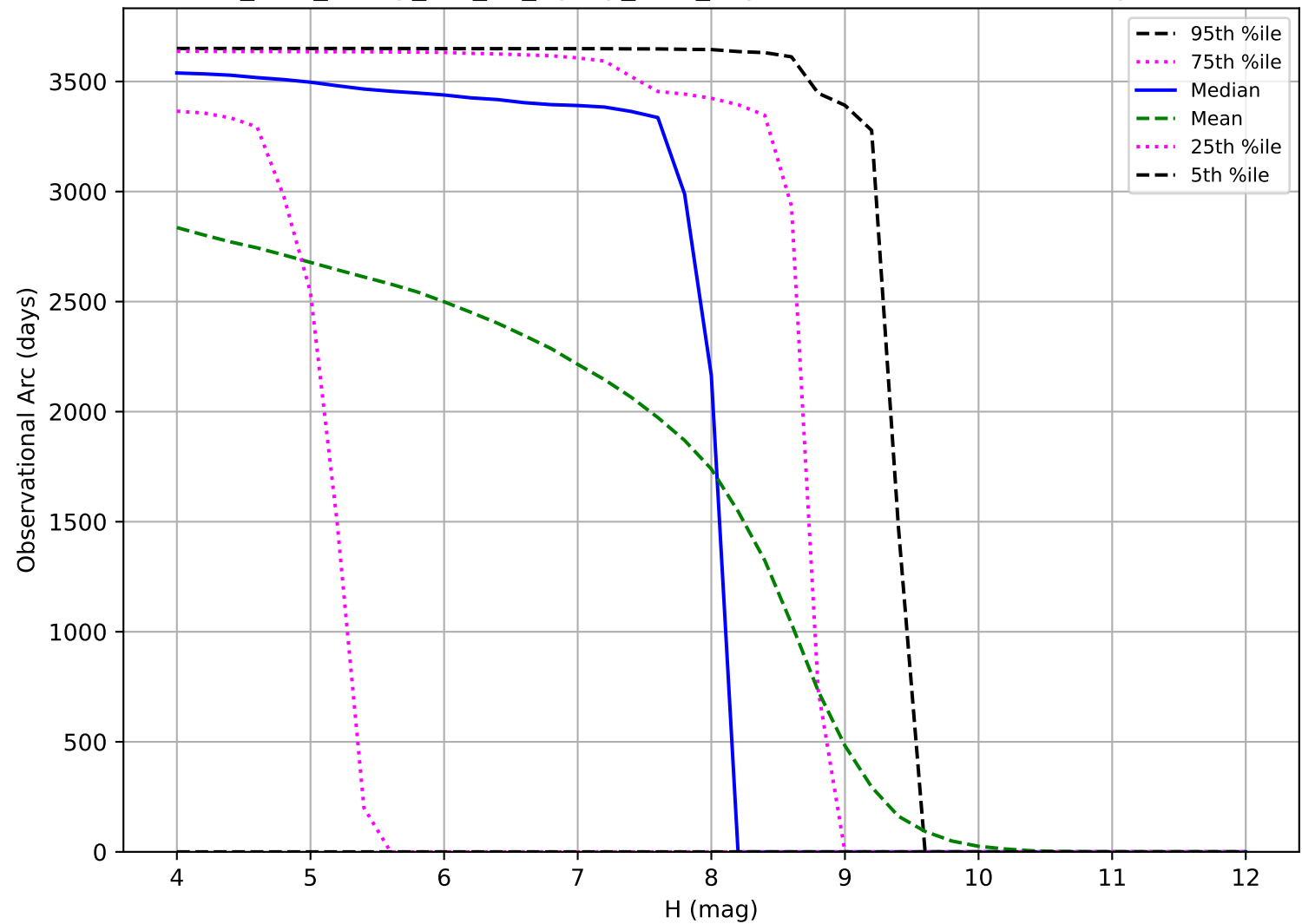
too_elab_heavy_r32_d2_ugrizy_v3.4_10yrs: Observational Arc Length TNO
