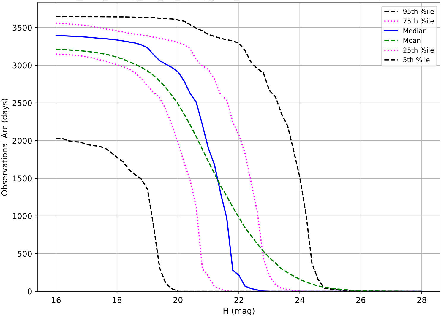
too_elab_heavy_r32_d2_ugrizy_v3.4_10yrs: Observational Arc Length PHA
