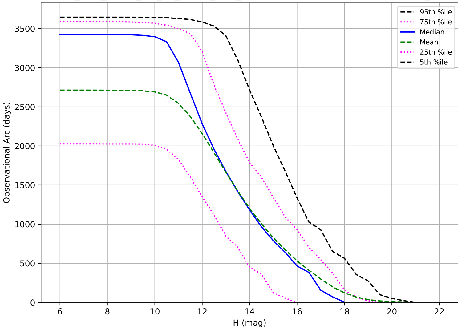
too_elab_heavy_r32_d2_ugrizy_v3.4_10yrs: Observational Arc Length OCC_r5
