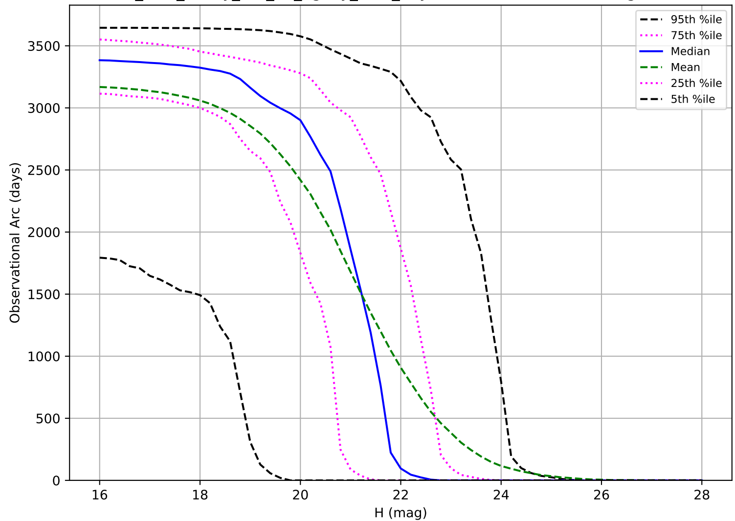
too_elab_heavy_r32_d2_ugrizy_v3.4_10yrs: Observational Arc Length NEO
