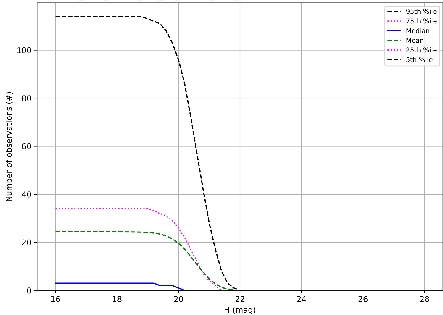
too_elab_heavy_r32_d2_ugrizy_v3.4_10yrs: Number of observations Vatira
