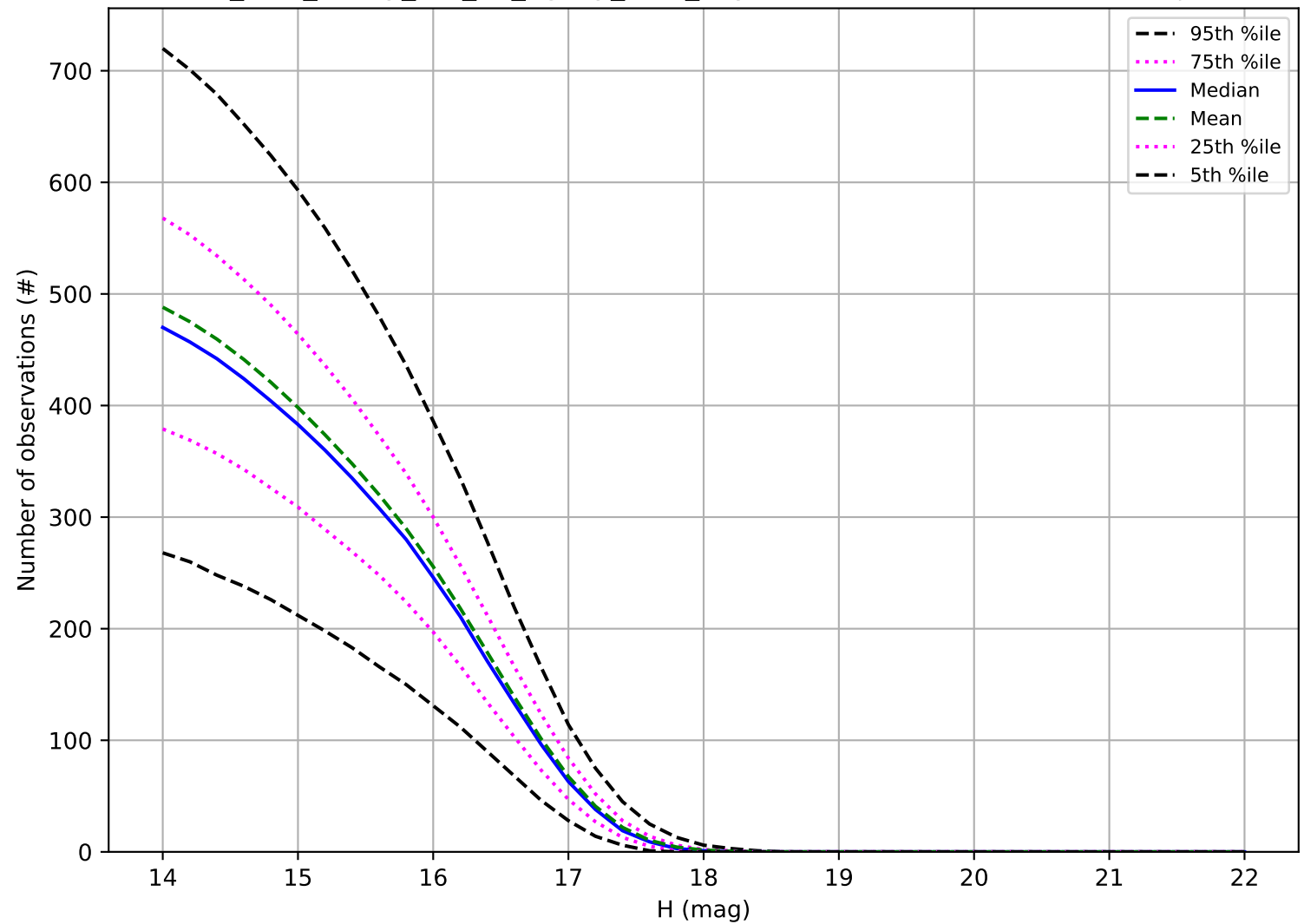
too_elab_heavy_r32_d2_ugrizy_v3.4_10yrs: Number of observations Trojan
