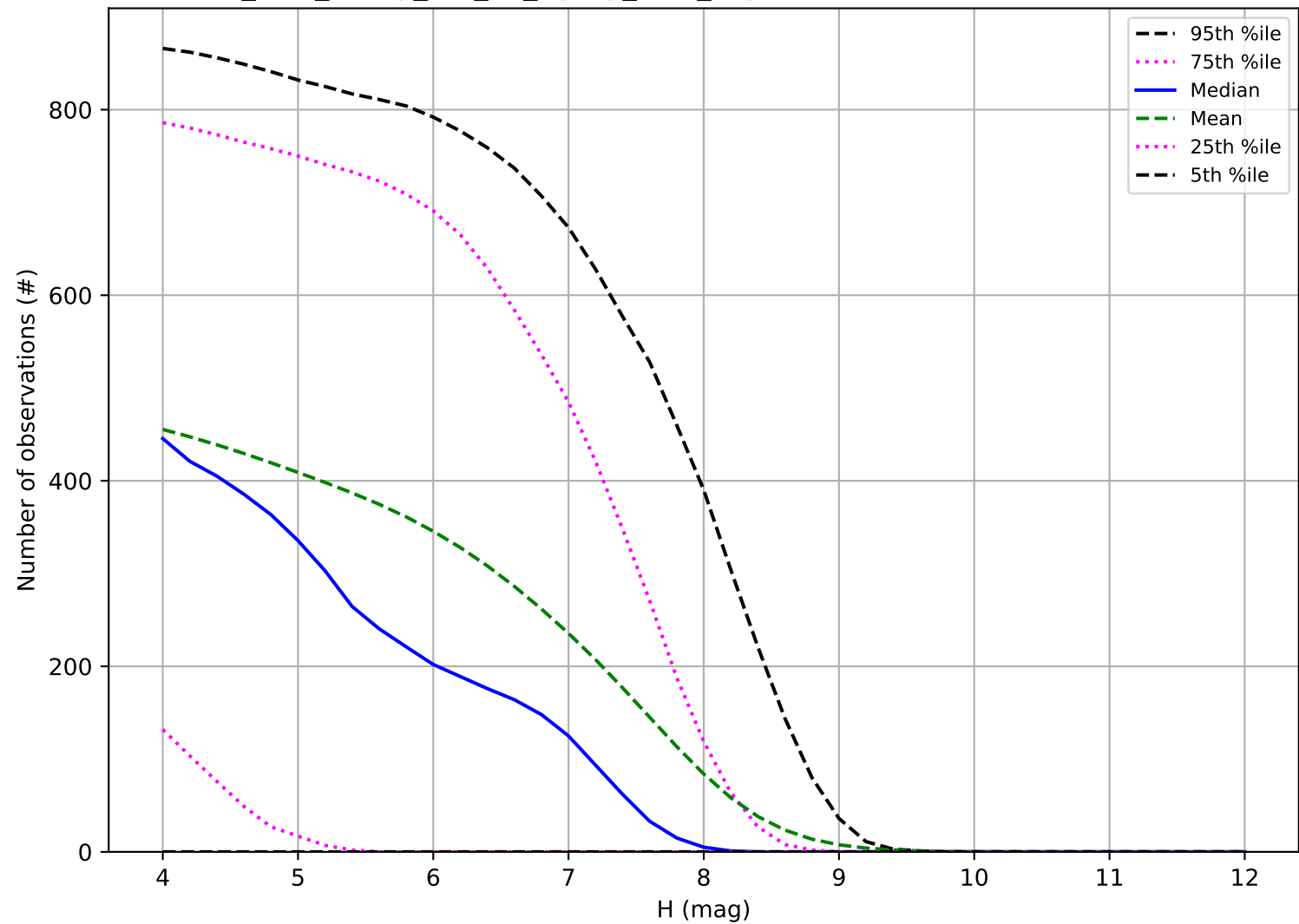
too_elab_heavy_r32_d2_ugrizy_v3.4_10yrs: Number of observations TNO
