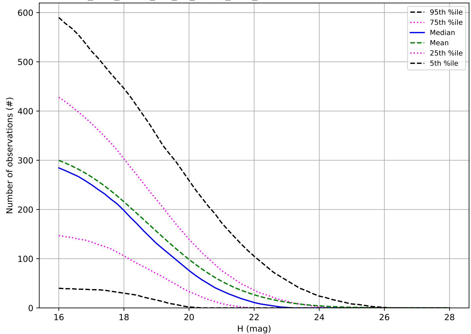
too_elab_heavy_r32_d2_ugrizy_v3.4_10yrs: Number of observations PHA
