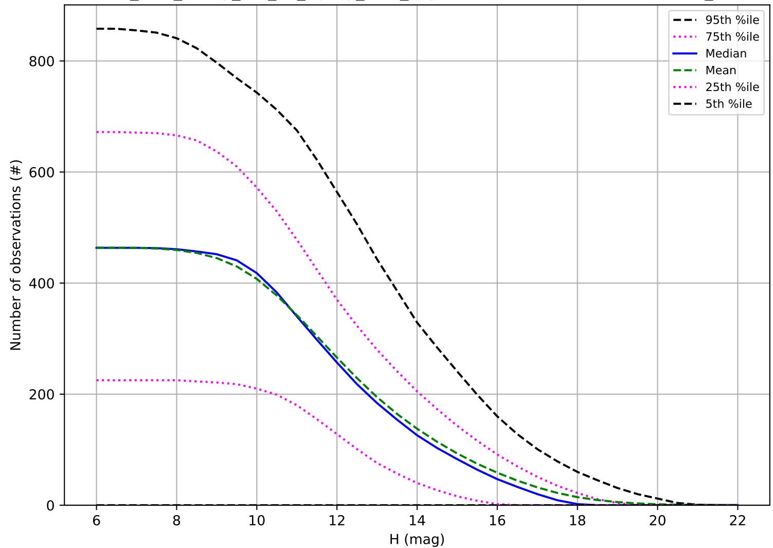
too_elab_heavy_r32_d2_ugrizy_v3.4_10yrs: Number of observations OCC_r5
