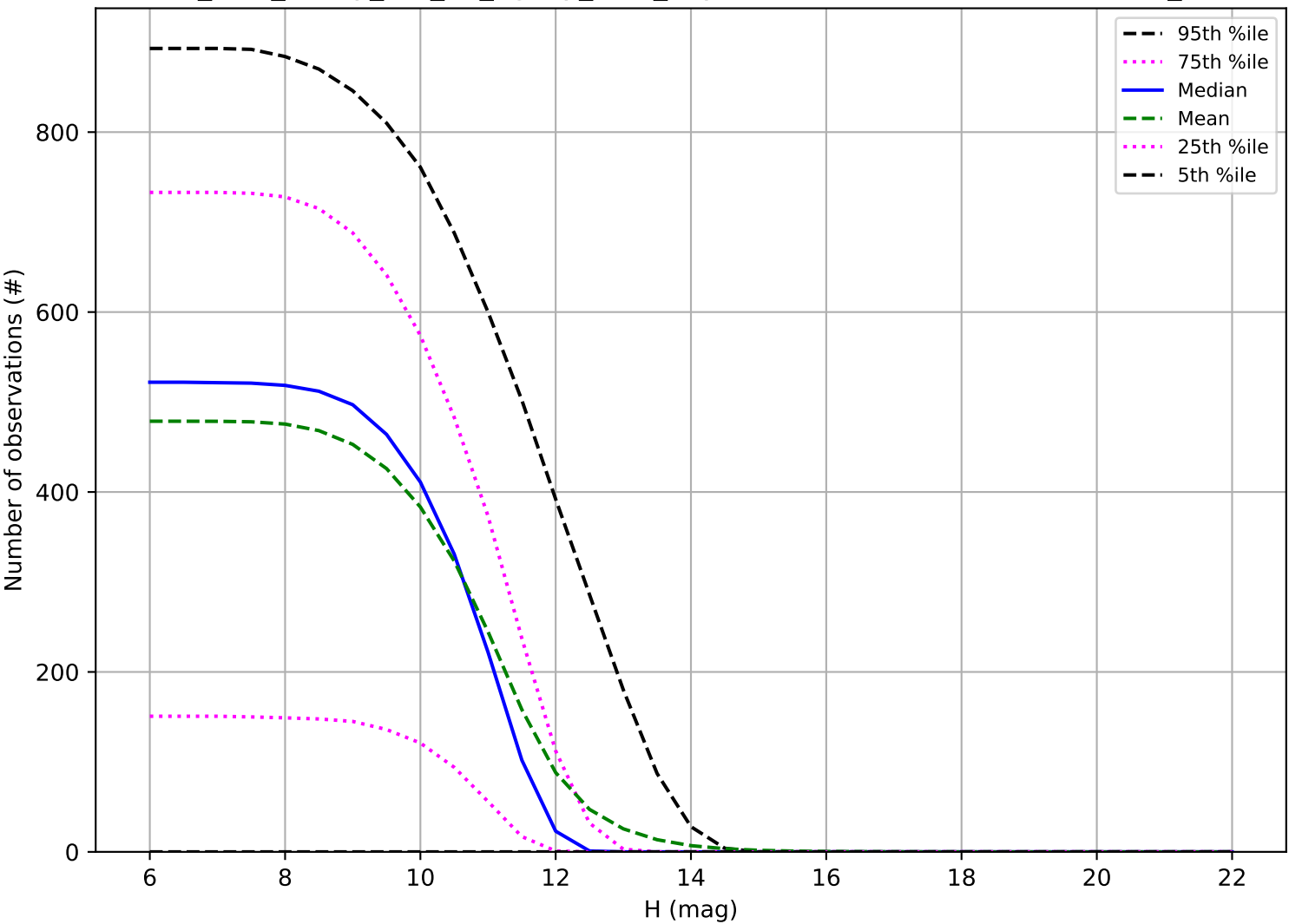
too_elab_heavy_r32_d2_ugrizy_v3.4_10yrs: Number of observations OCC_r20
