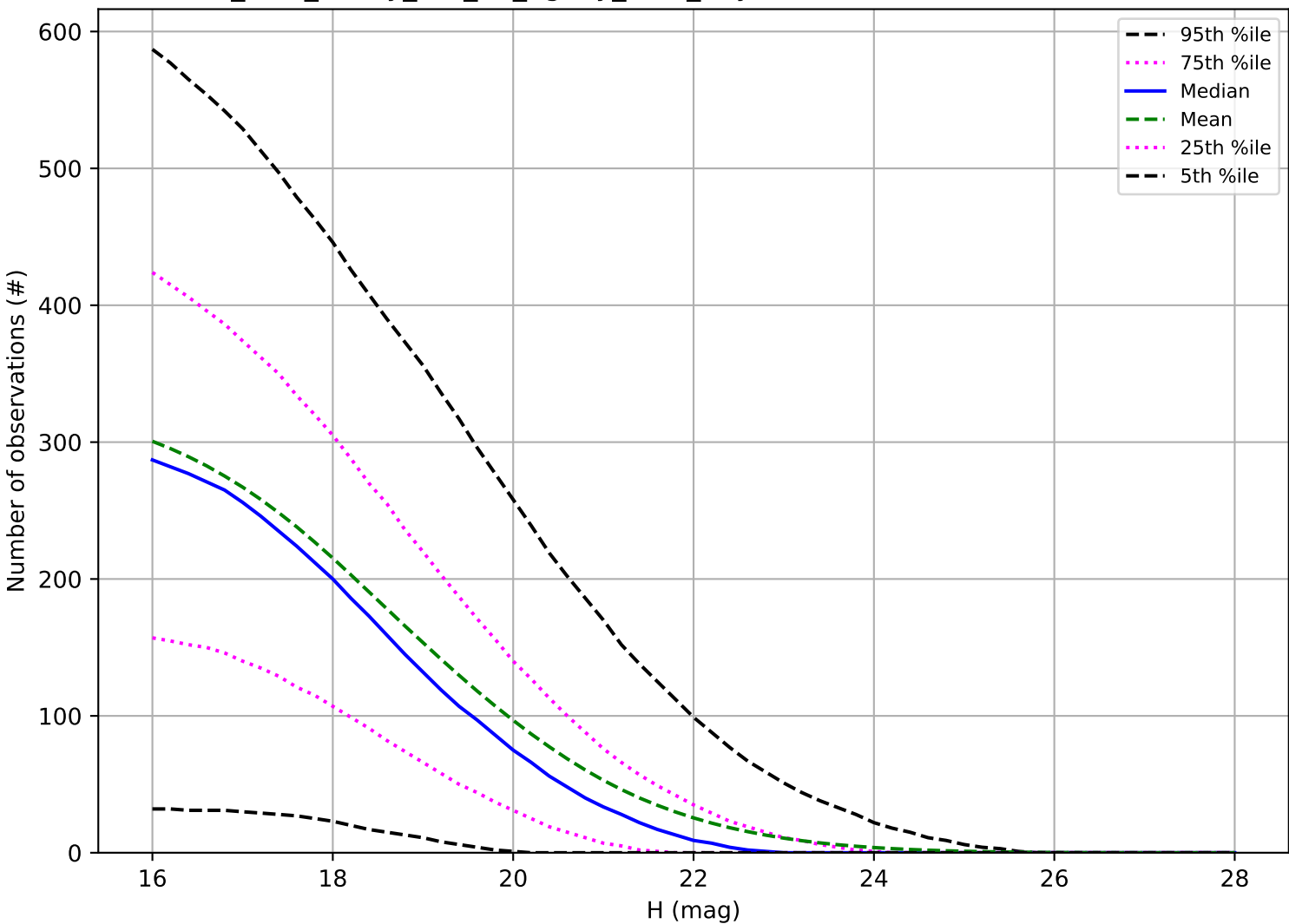
too_elab_heavy_r32_d2_ugrizy_v3.4_10yrs: Number of observations NEO
