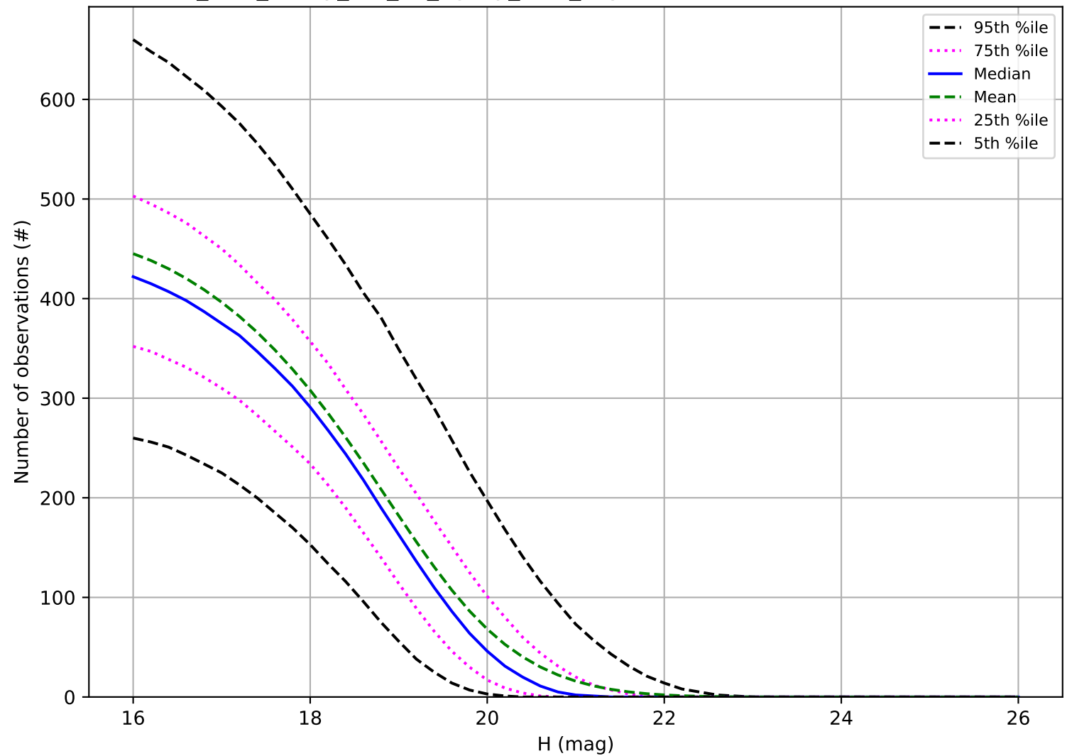
too_elab_heavy_r32_d2_ugrizy_v3.4_10yrs: Number of observations MBA
