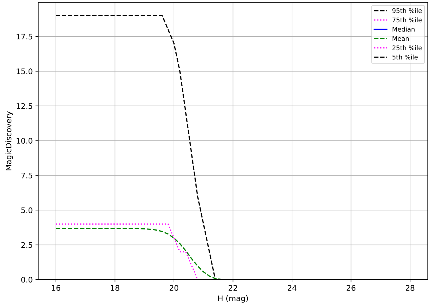
too_elab_heavy_r32_d2_ugrizy_v3.4_10yrs: Vatira 6 detections in 60 nights detection loss
