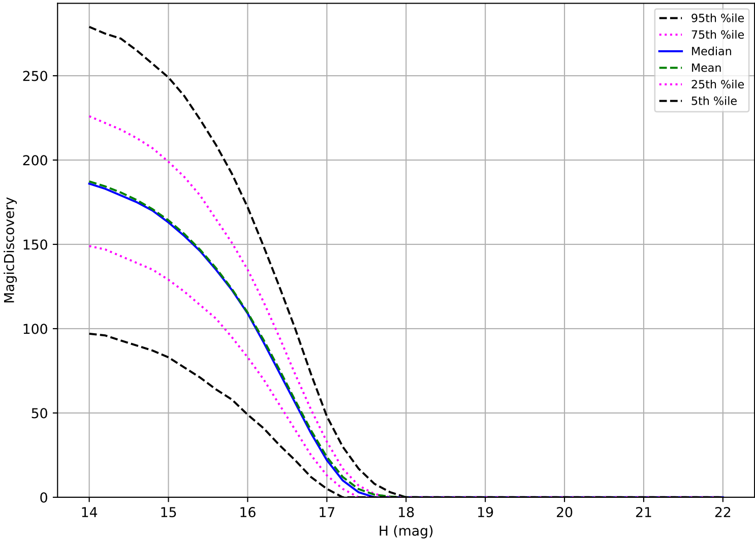
too_elab_heavy_r32_d2_ugrizy_v3.4_10yrs: Trojan 6 detections in 60 nights detection loss
