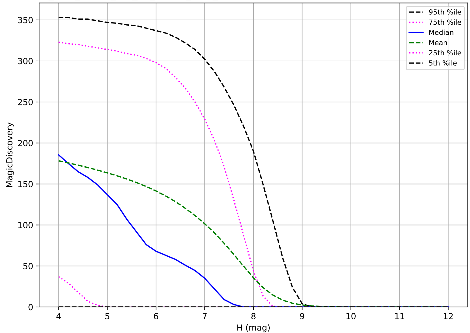
too_elab_heavy_r32_d2_ugrizy_v3.4_10yrs: TNO 6 detections in 60 nights detection loss
