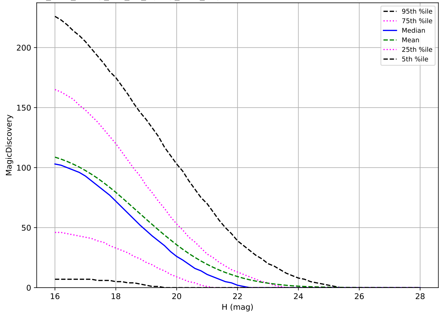
too_elab_heavy_r32_d2_ugrizy_v3.4_10yrs: PHA 6 detections in 60 nights detection loss
