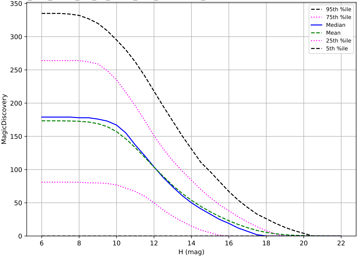
too_elab_heavy_r32_d2_ugrizy_v3.4_10yrs: OCC_r5 6 detections in 60 nights detection loss
