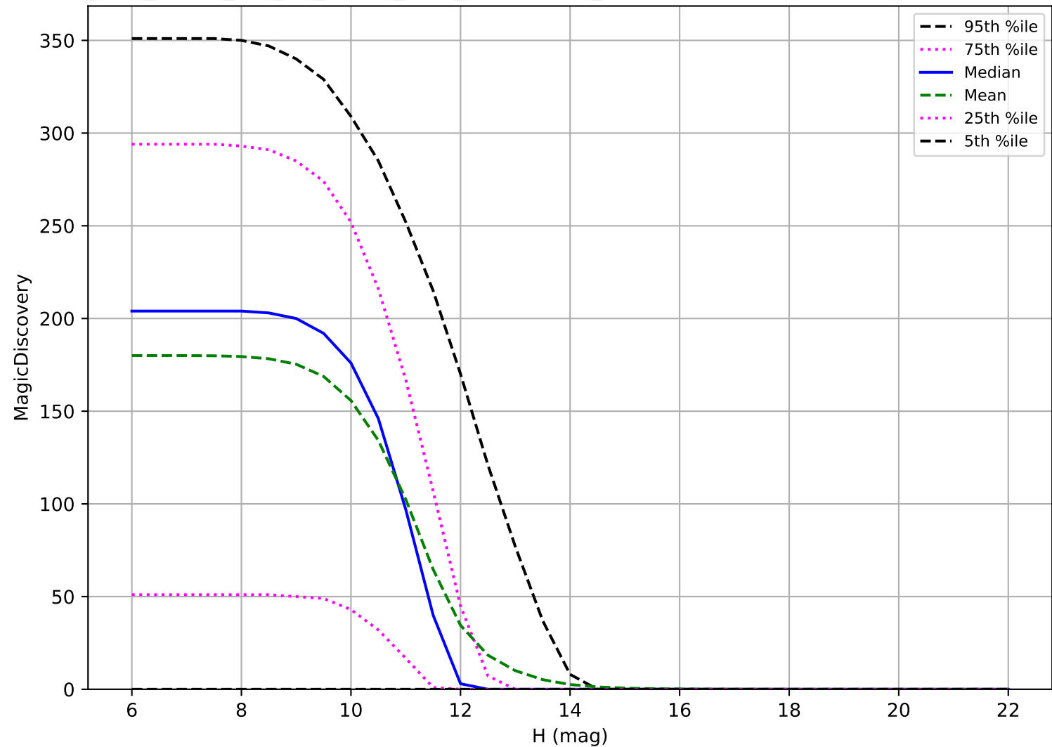
too_elab_heavy_r32_d2_ugrizy_v3.4_10yrs: OCC_r20 6 detections in 60 nights detection loss
