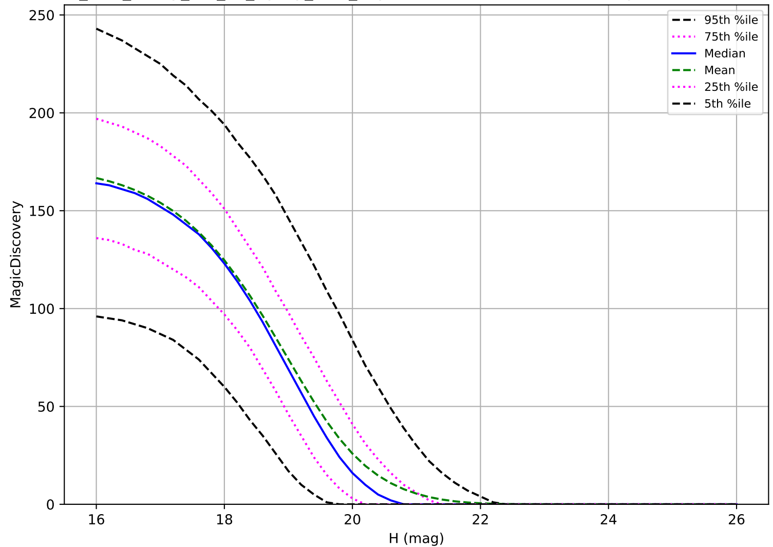
too_elab_heavy_r32_d2_ugrizy_v3.4_10yrs: MBA 6 detections in 60 nights detection loss
