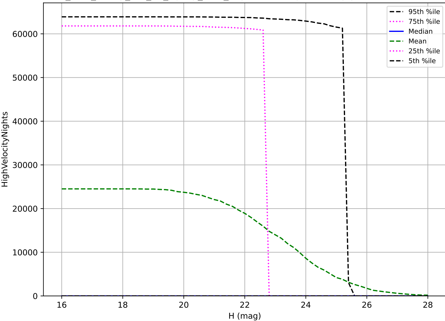
too_elab_heavy_r32_d2_ugrizy_v3.4_10yrs: PHA High velocity pair detection loss
