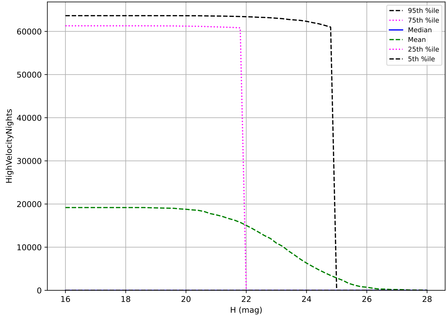
too_elab_heavy_r32_d2_ugrizy_v3.4_10yrs: NEO High velocity pair detection loss
