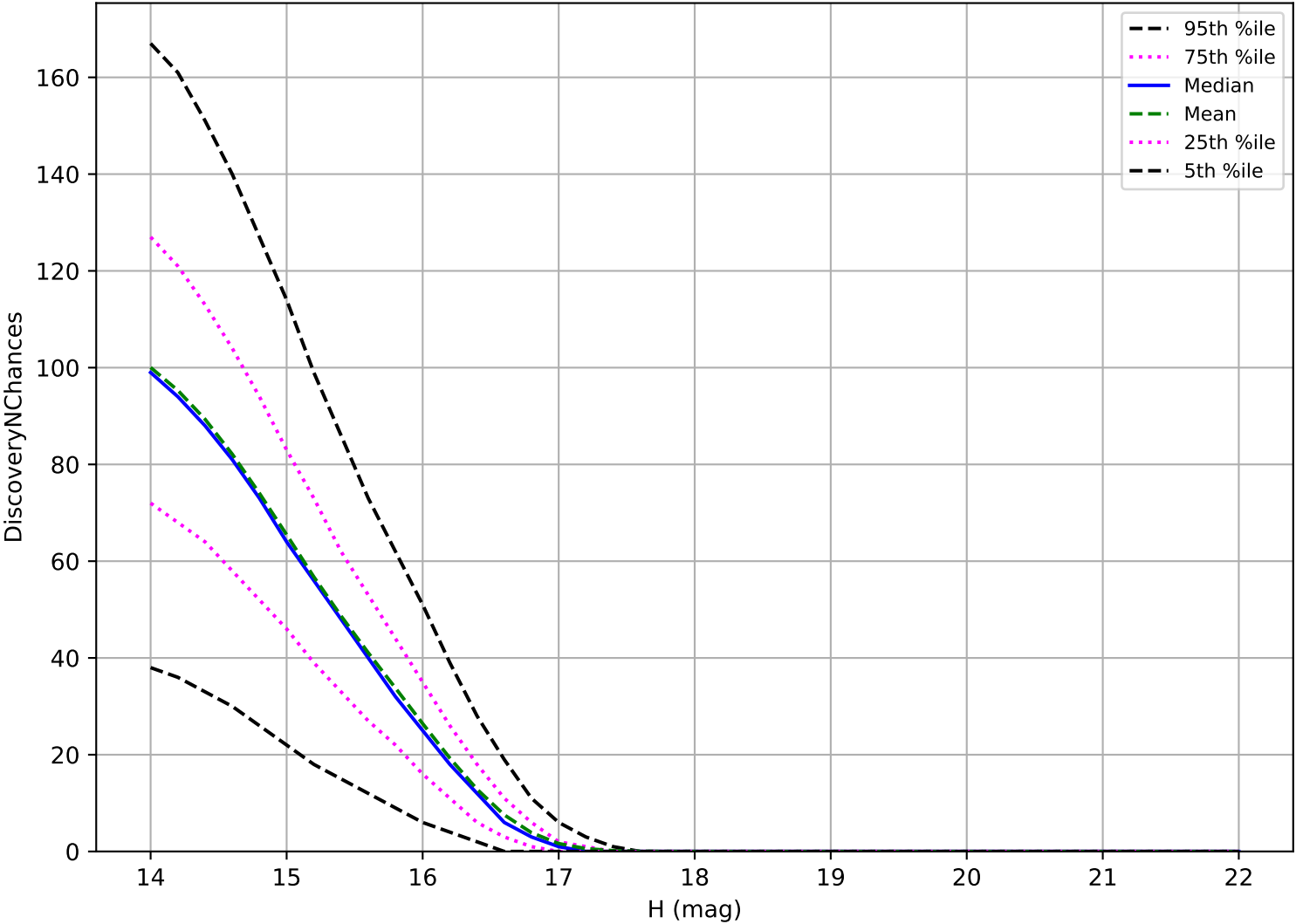
too_elab_heavy_r32_d2_ugrizy_v3.4_10yrs: Trojan 3 pairs in 15 nights detection loss
