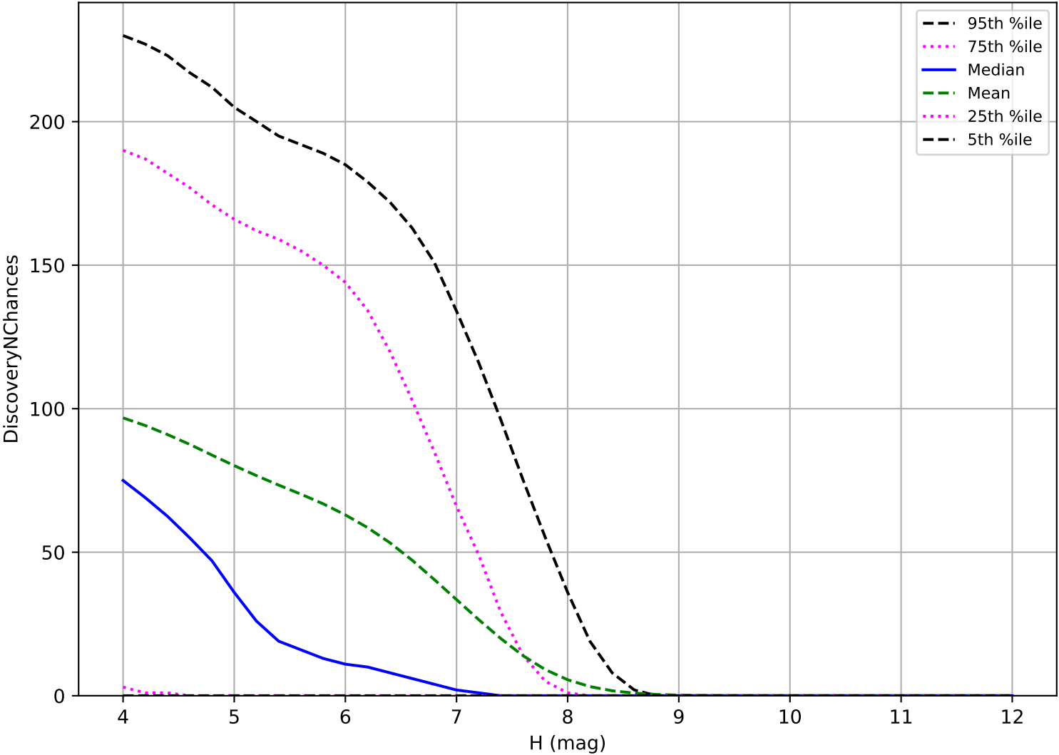
too_elab_heavy_r32_d2_ugrizy_v3.4_10yrs: TNO 3 pairs in 15 nights detection loss
