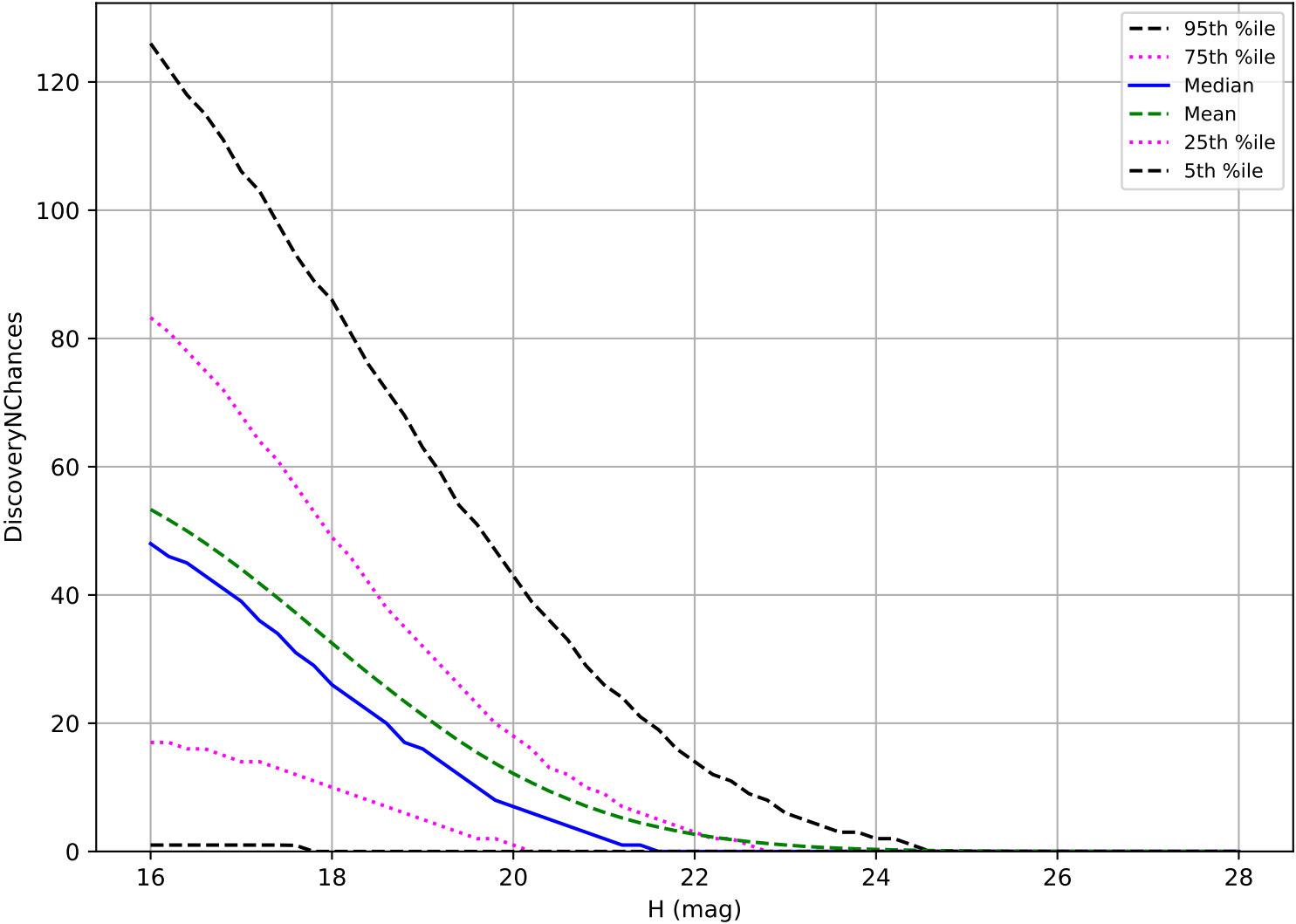
too_elab_heavy_r32_d2_ugrizy_v3.4_10yrs: PHA 3 pairs in 15 nights detection loss
