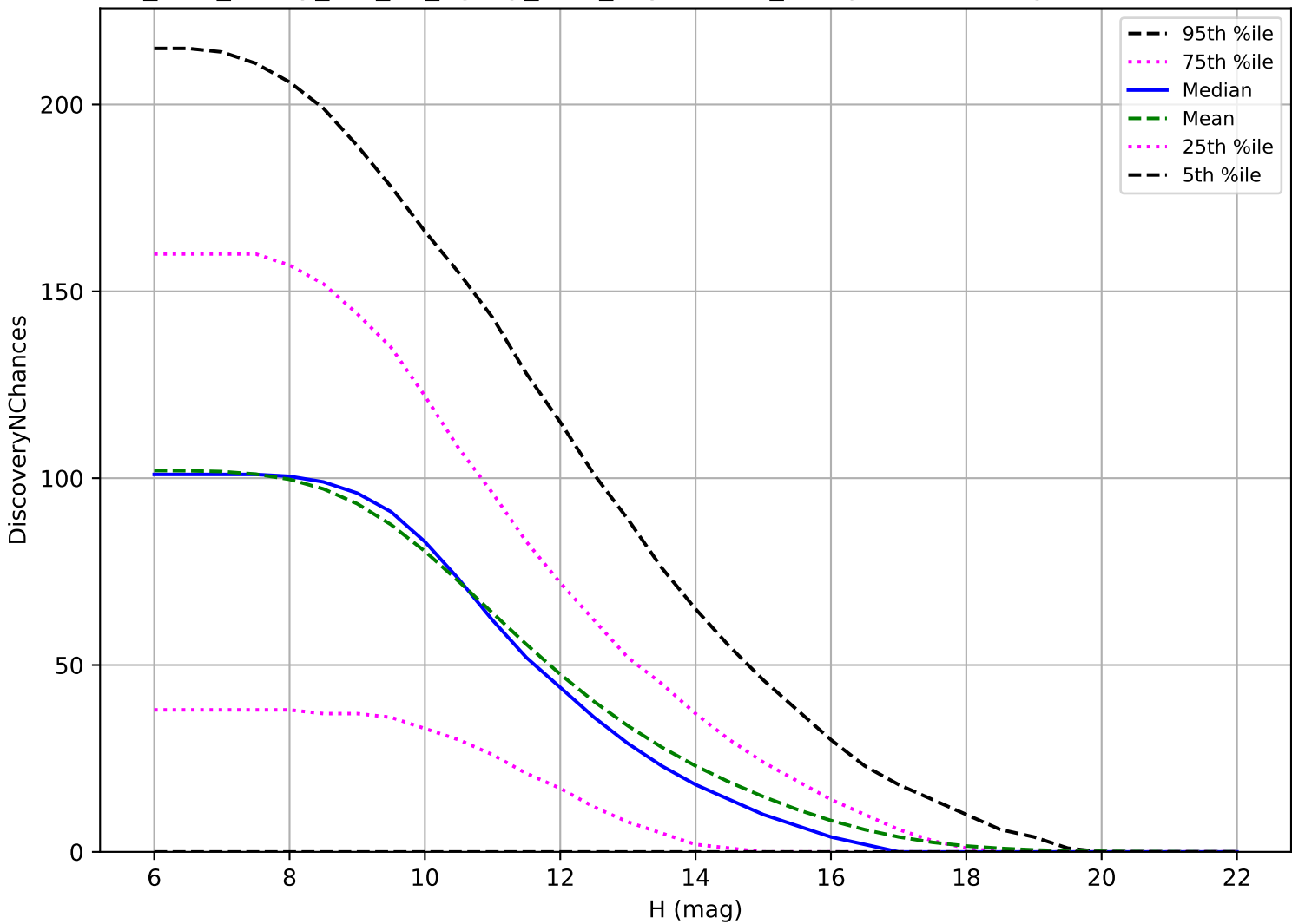
too_elab_heavy_r32_d2_ugrizy_v3.4_10yrs: OCC_r5 3 pairs in 15 nights detection loss
