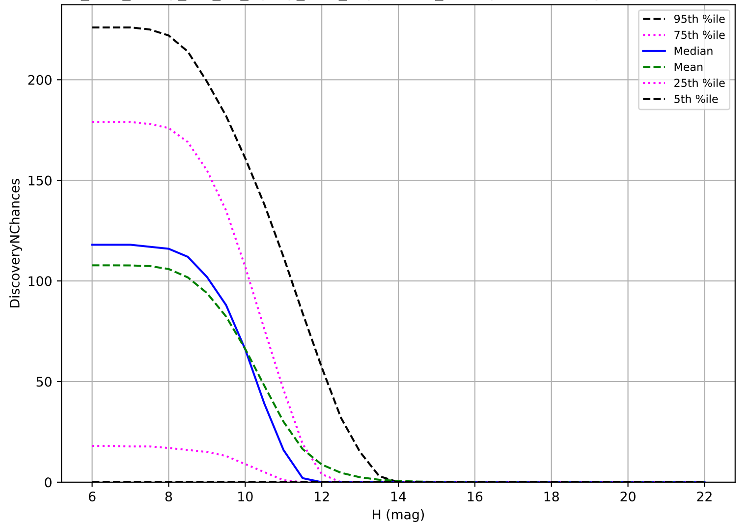
too_elab_heavy_r32_d2_ugrizy_v3.4_10yrs: OCC_r20 3 pairs in 15 nights detection loss
