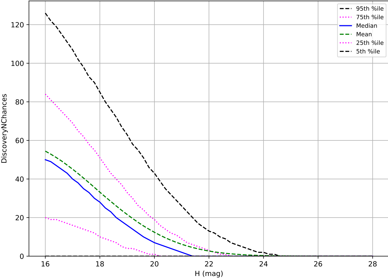
too_elab_heavy_r32_d2_ugrizy_v3.4_10yrs: NEO 3 pairs in 15 nights detection loss
