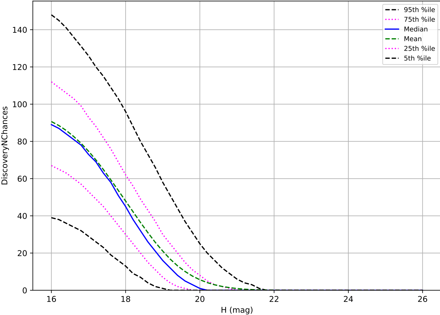
too_elab_heavy_r32_d2_ugrizy_v3.4_10yrs: MBA 3 pairs in 15 nights detection loss
