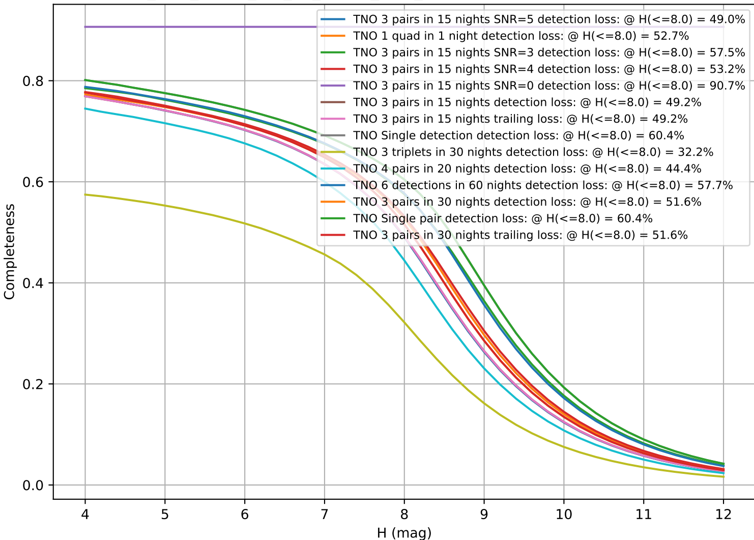
too_elab_heavy_r32_d2_ugrizy_v3.4_10yrs: CumulativeCompleteness
