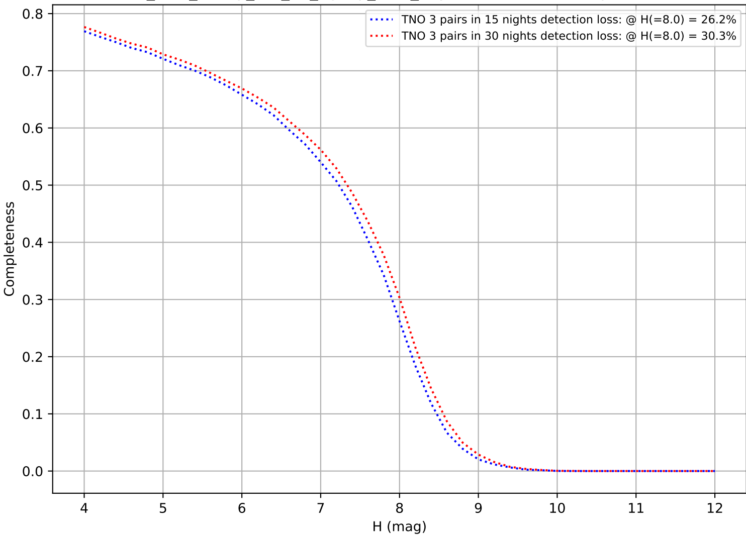
too_elab_heavy_r32_d2_ugrizy_v3.4_10yrs: DifferentialCompleteness
