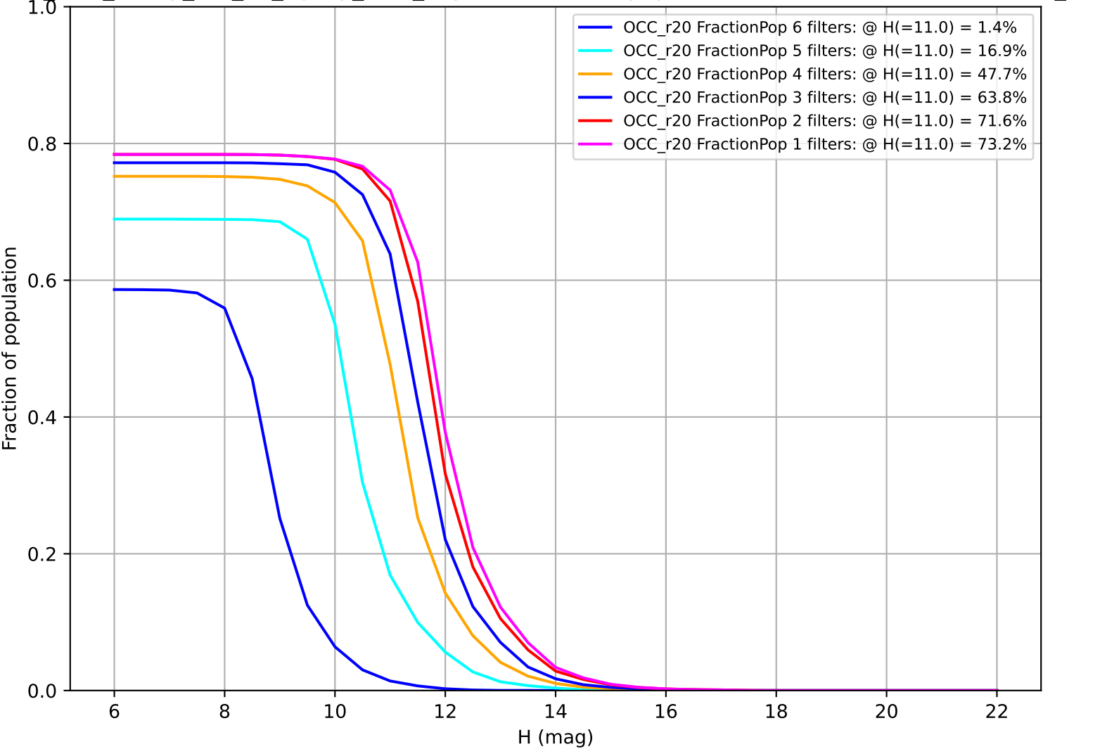
too_elab_heavy_r32_d2_ugrizy_v3.4_10yrs: Fraction of population with colors in X filters OCC_r20
