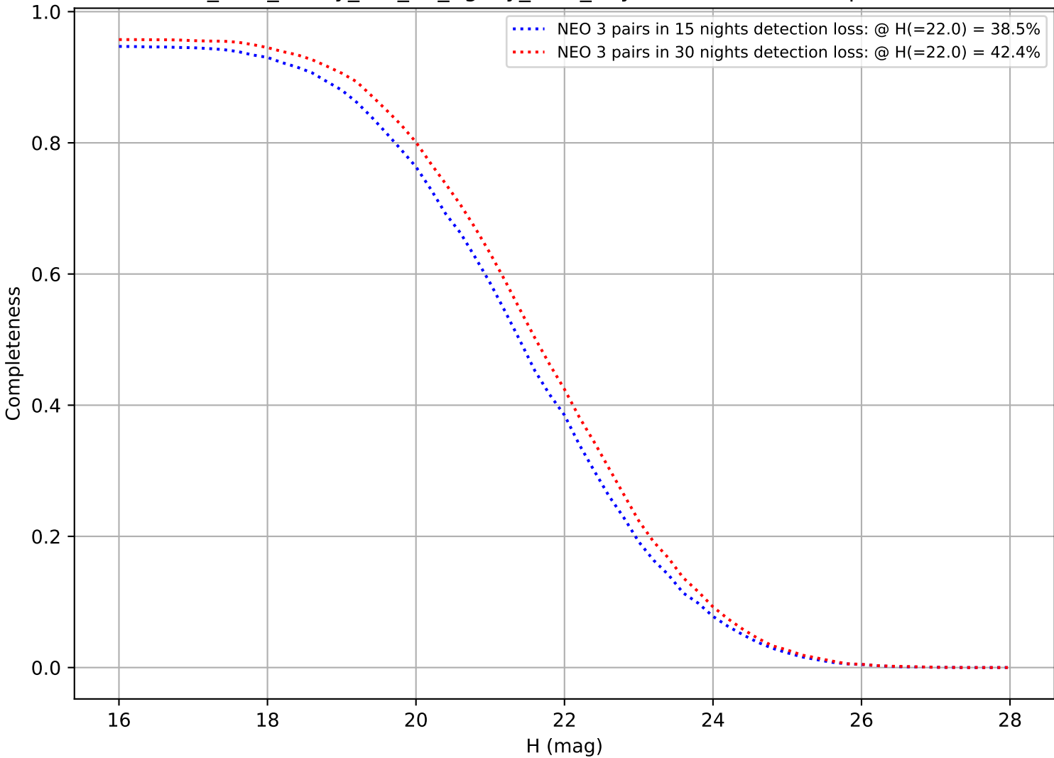
too_elab_heavy_r32_d2_ugrizy_v3.4_10yrs: DifferentialCompleteness
