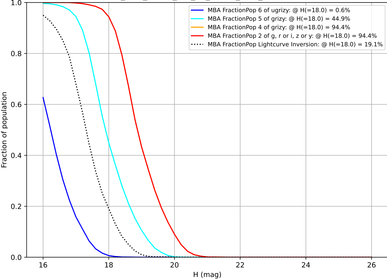
too_elab_heavy_r32_d2_ugrizy_v3.4_10yrs MBA
