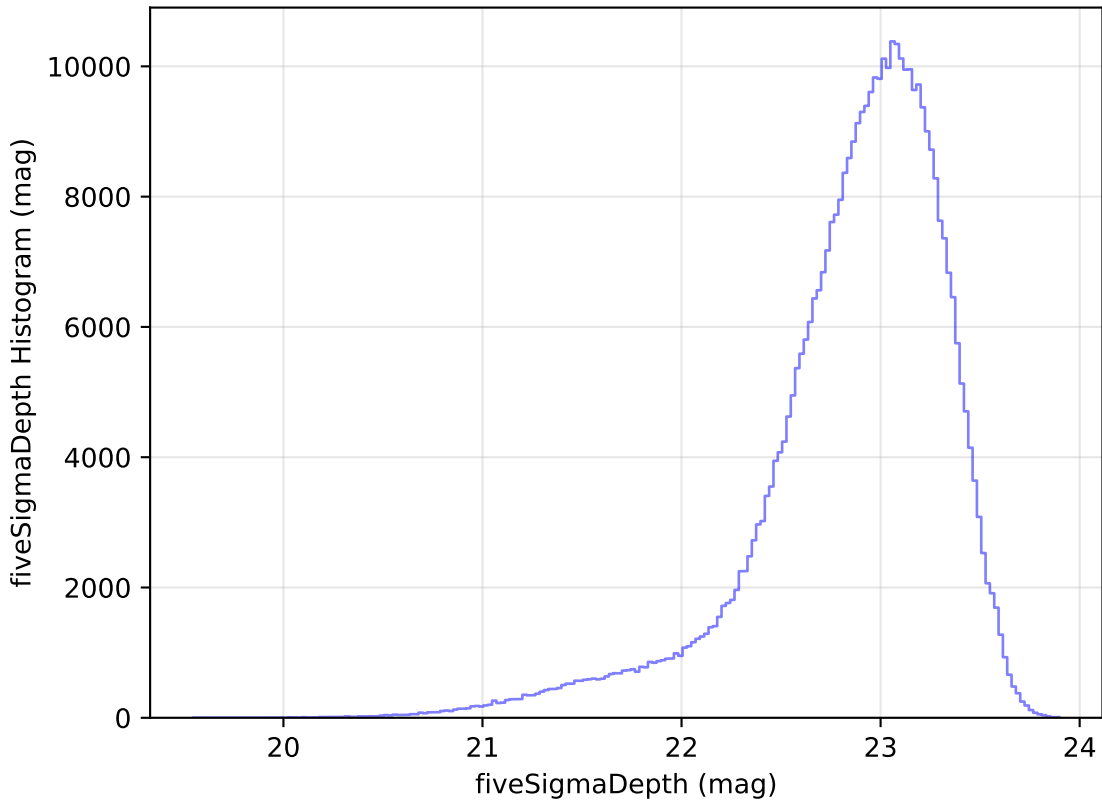
too_elab_heavy_r32_d2_ugrizy_v3.4_10yrs z: fiveSigmaDepth Histogram
