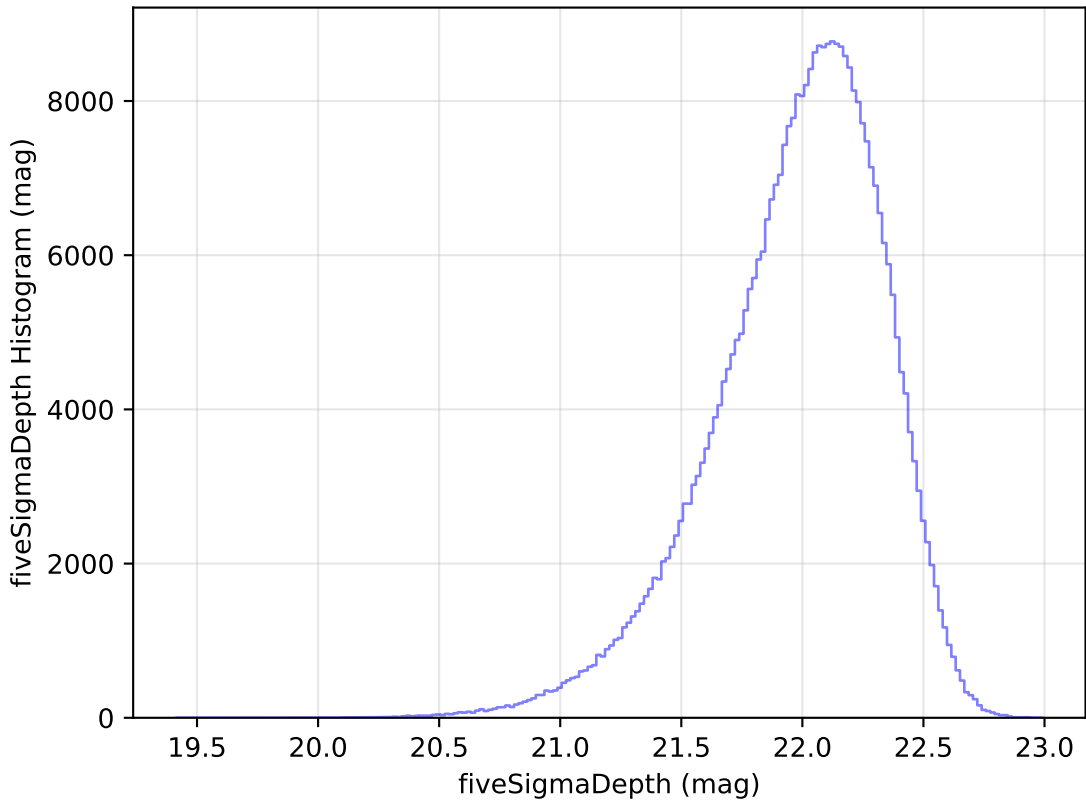
too_elab_heavy_r32_d2_ugrizy_v3.4_10yrs y: fiveSigmaDepth Histogram
