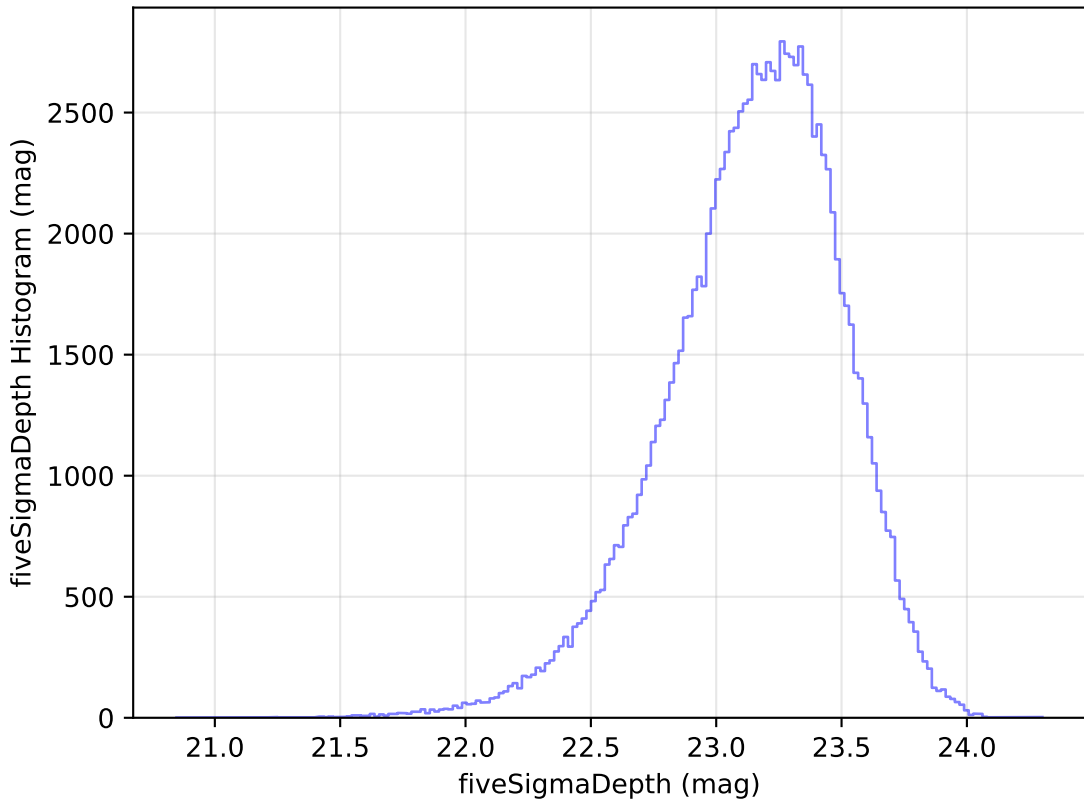
too_elab_heavy_r32_d2_ugrizy_v3.4_10yrs u: fiveSigmaDepth Histogram
