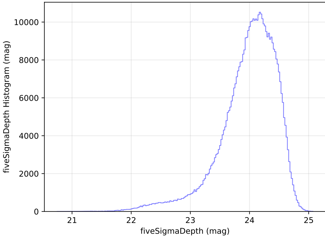
too_elab_heavy_r32_d2_ugrizy_v3.4_10yrs r: fiveSigmaDepth Histogram
