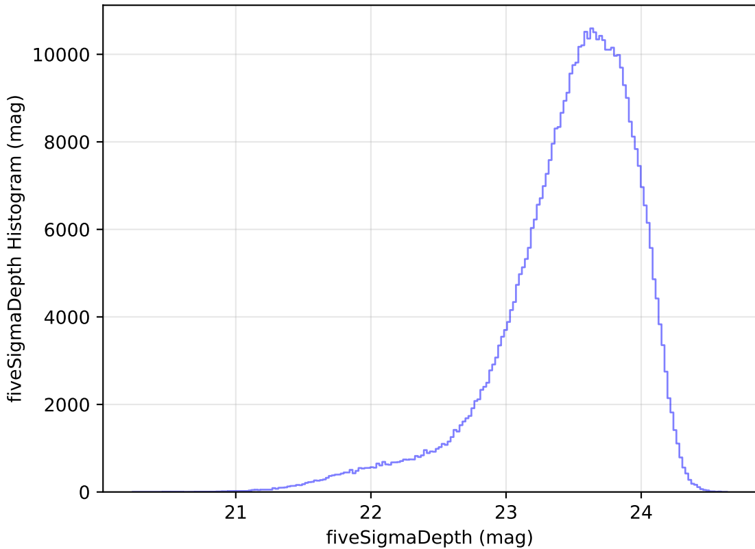
too_elab_heavy_r32_d2_ugrizy_v3.4_10yrs i: fiveSigmaDepth Histogram
