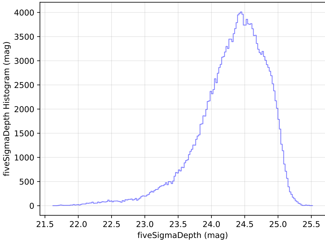
too_elab_heavy_r32_d2_ugrizy_v3.4_10yrs g: fiveSigmaDepth Histogram
