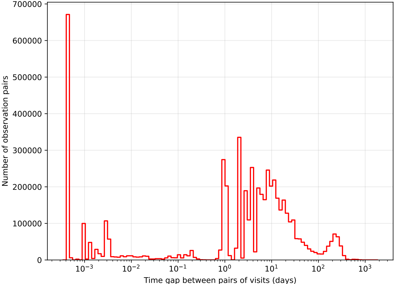
too_elab_heavy_r32_d2_ugrizy_v3.4_10yrs i band: Tgaps observationStartMJD
