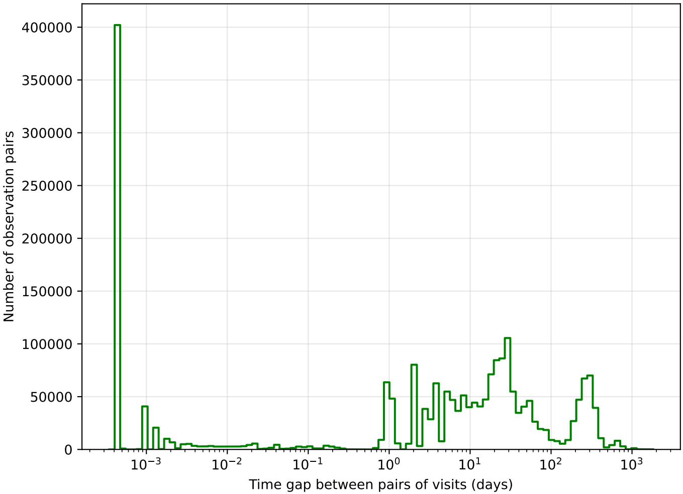
too_elab_heavy_r32_d2_ugrizy_v3.4_10yrs g band: Tgaps observationStartMJD
