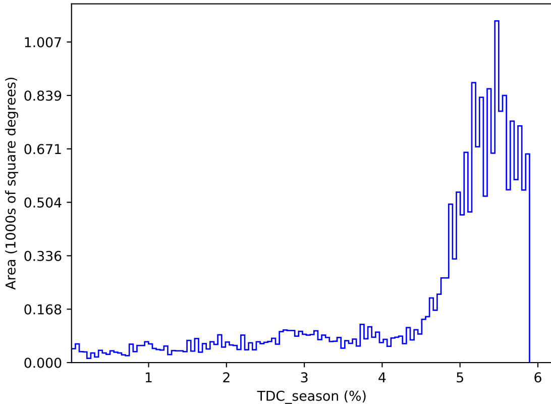
too_elab_heavy_r32_d2_ugrizy_v3.4_10yrs : TDC_season
