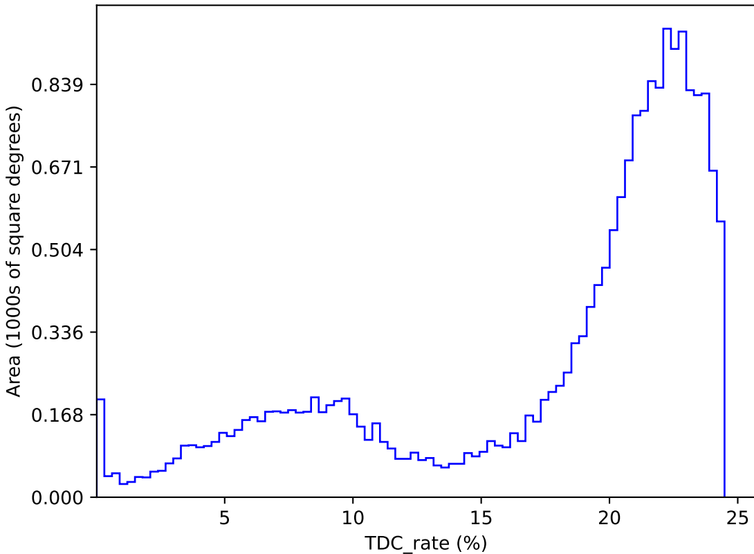
too_elab_heavy_r32_d2_ugrizy_v3.4_10yrs : TDC_rate
