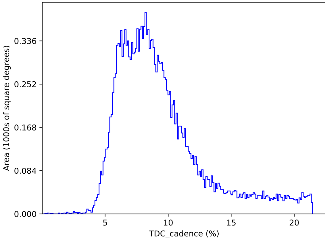
too_elab_heavy_r32_d2_ugrizy_v3.4_10yrs : TDC_cadence
