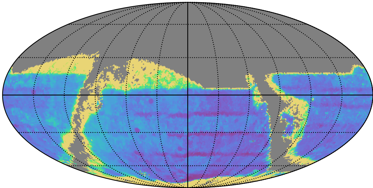
too_elab_heavy_r32_d2_ugrizy_v3.4_10yrs : TDC_accuracy
