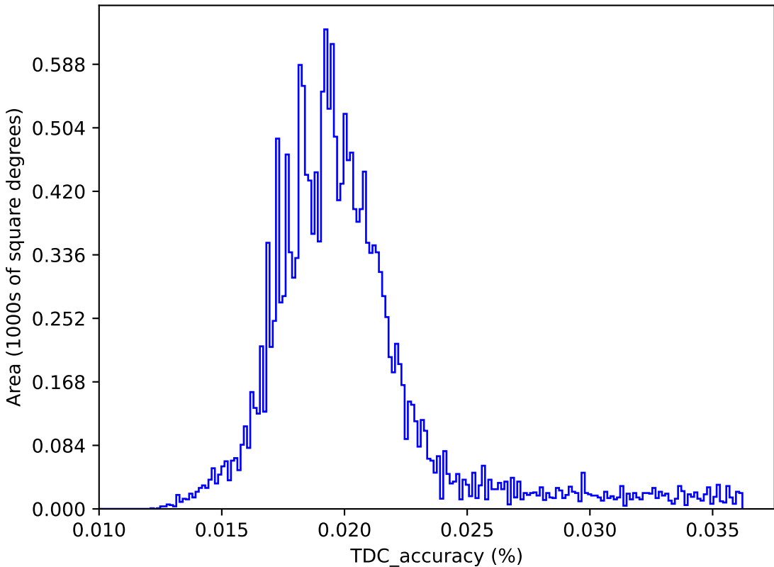
too_elab_heavy_r32_d2_ugrizy_v3.4_10yrs : TDC_accuracy
