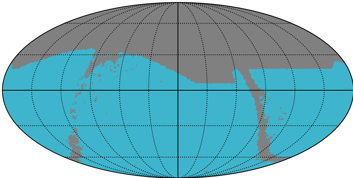
too_elab_heavy_r32_d2_ugrizy_v3.4_10yrs : SNSLMetric
