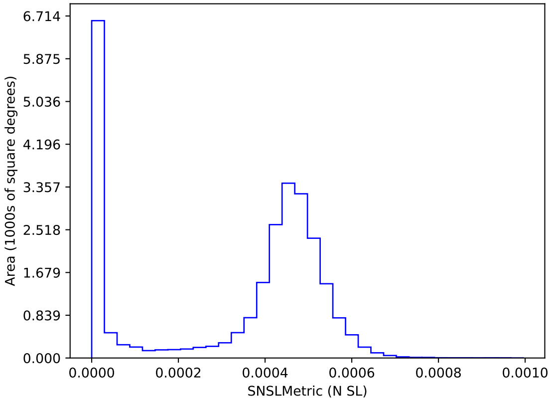
too_elab_heavy_r32_d2_ugrizy_v3.4_10yrs : SNSLMetric
