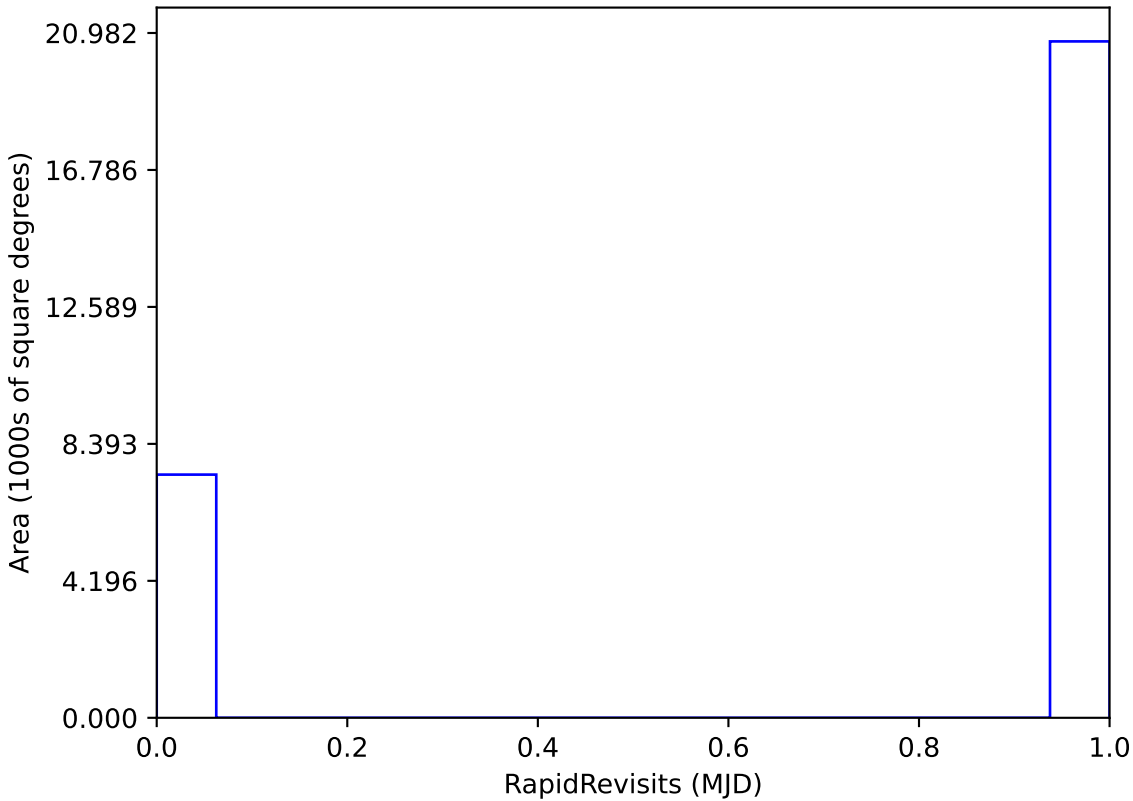
too_elab_heavy_r32_d2_ugrizy_v3.4_10yrs : RapidRevisits
